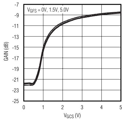
SMALL-SIGNAL GAIN vs. V_GCS
